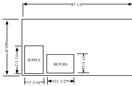
EXISTING UNIT
